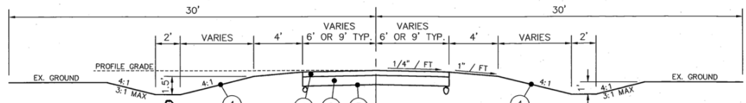
COMMON ACCESS DRIVE TYPICAL SECTION
