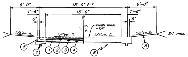
TYPICAL ACCESS DRIVE PAVEMENT SECTION
